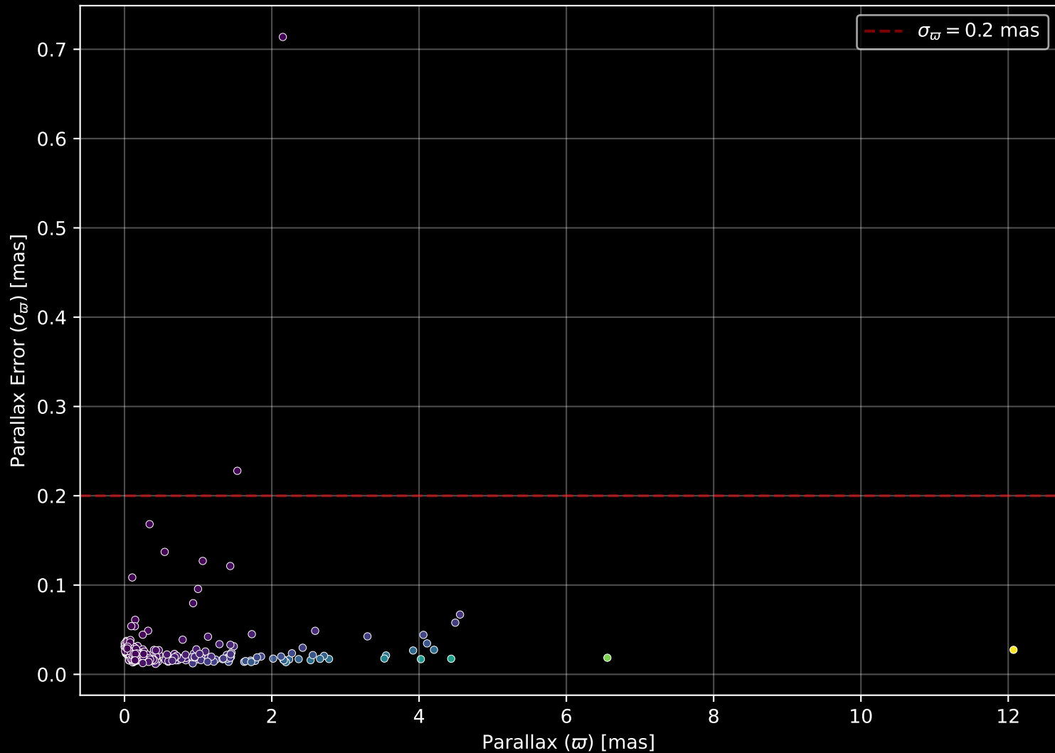
APOGEE DR17 Field: [SGRC3] Parallax Quality (n= 308)
