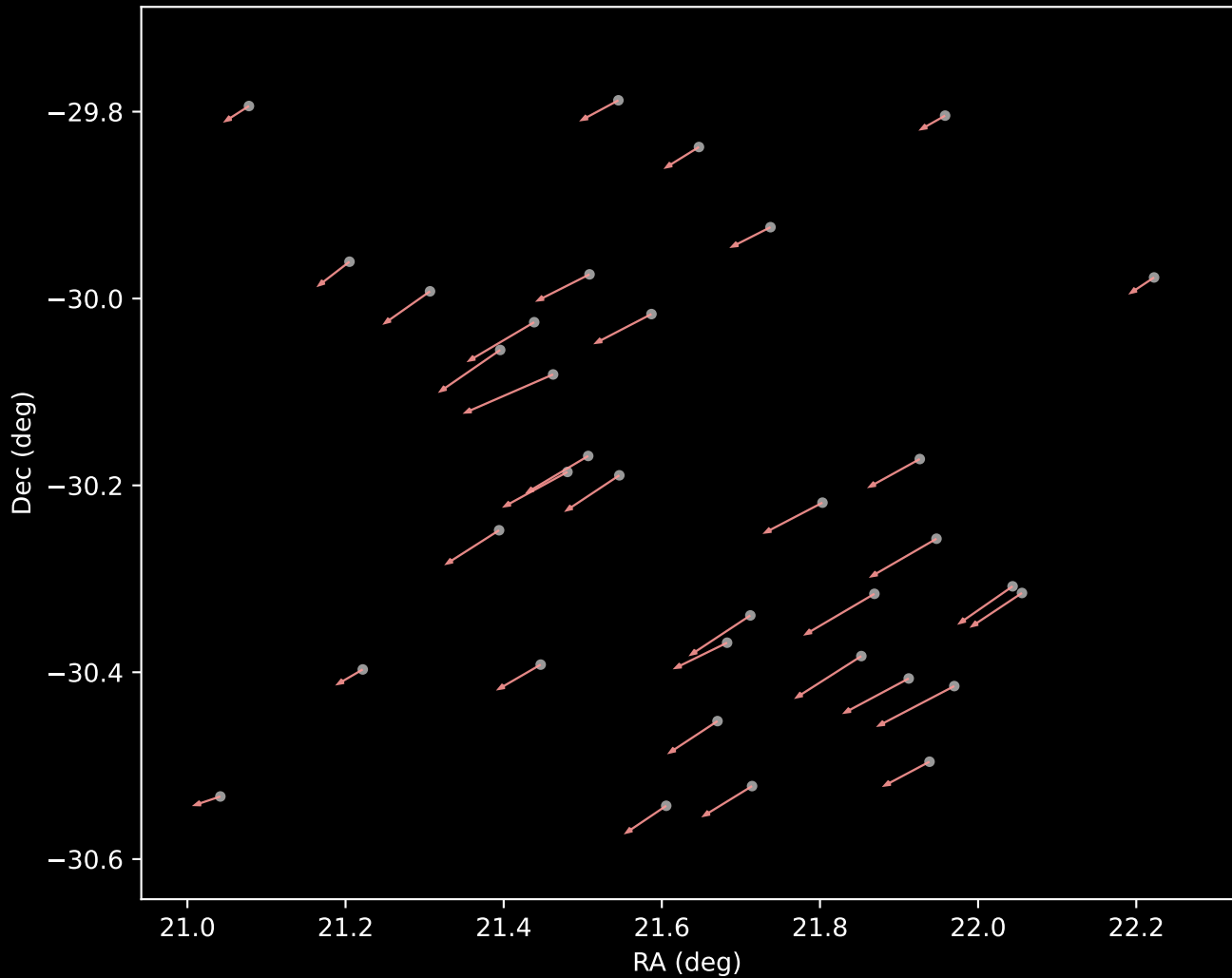
APOGEE DR17 Cluster 7 Proper Motion Vectors (n=35)
