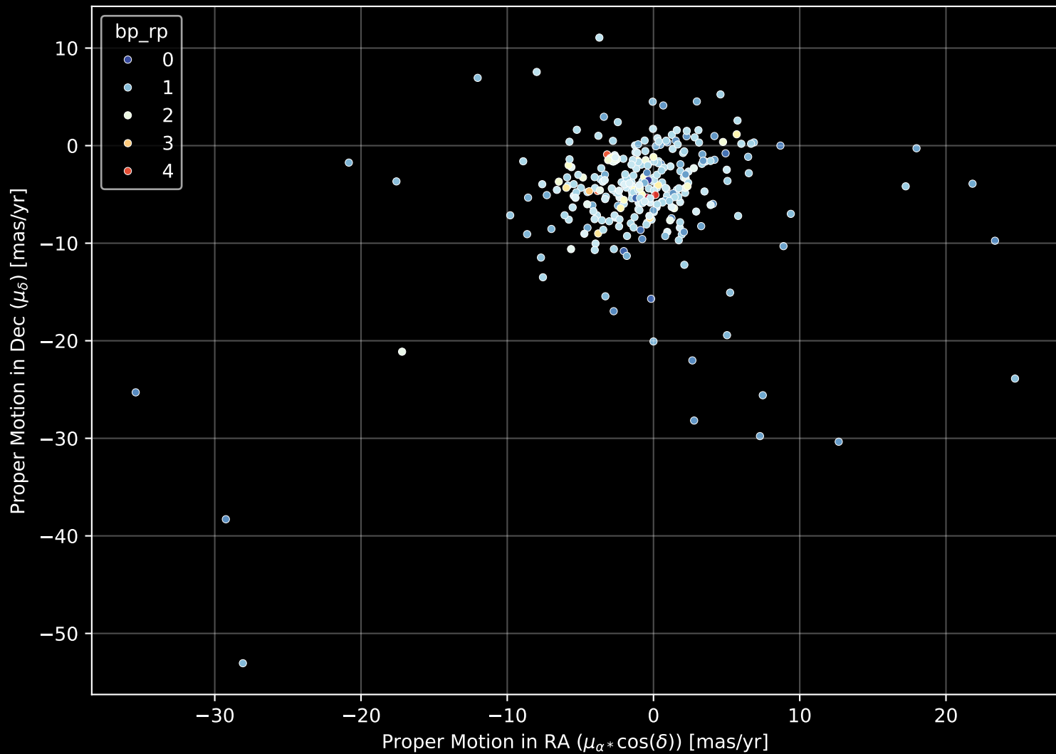
APOGEE DR17 Field: [SGRC3] Proper Motion Diagram (n= 308)
