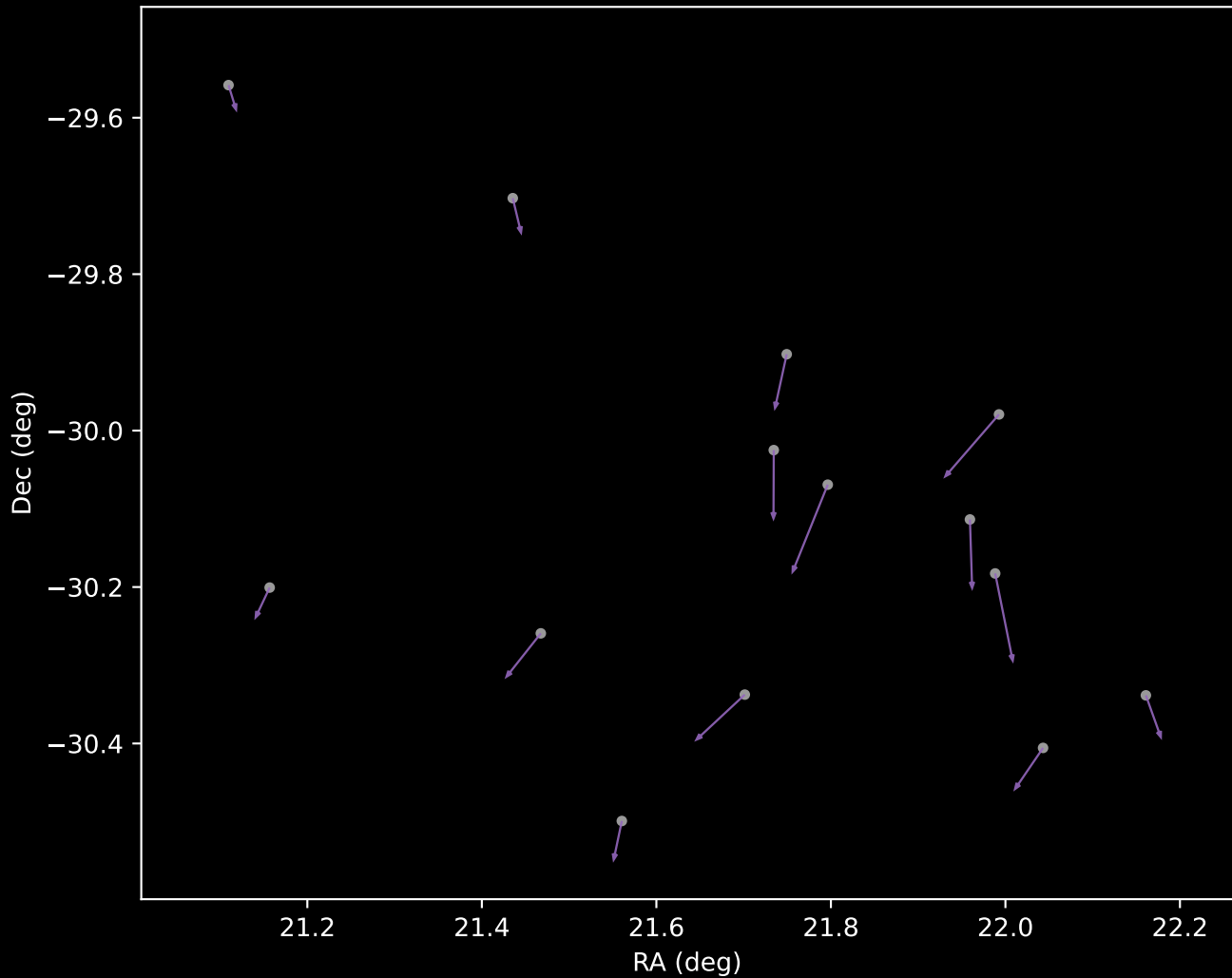
APOGEE DR17 Cluster 8 Proper Motion Vectors (n=14)
