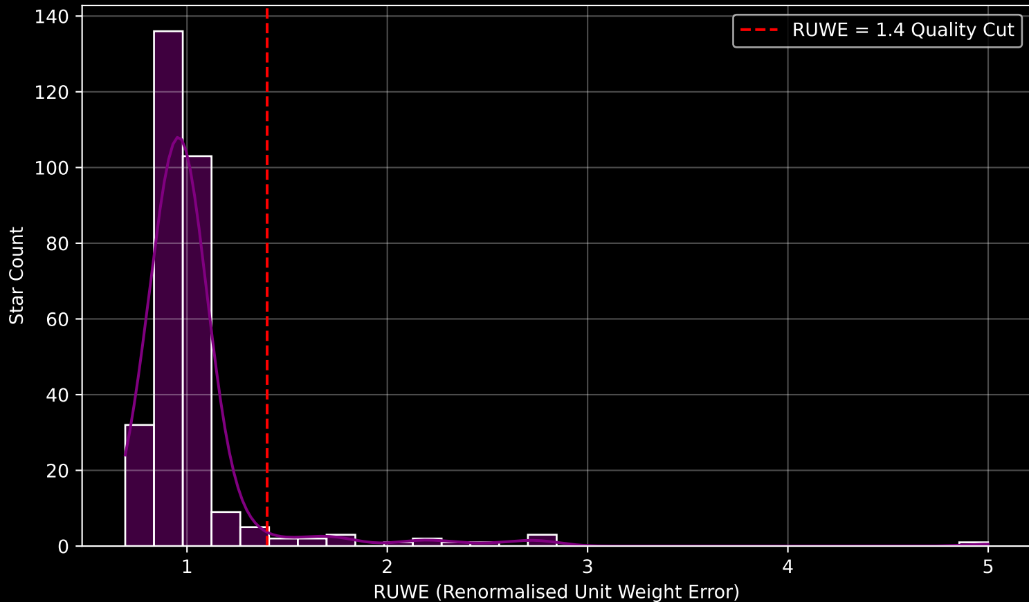
GAPOGEE DR17 Field [SGRC3] RUWE Distribution (n= 301)
