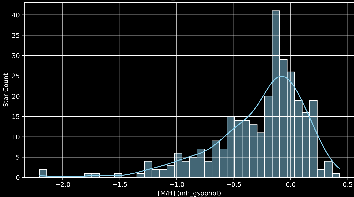
APOGEE DR17 Field: [SGRC3 [M/H] (mh_gspphot) (n= 303)
