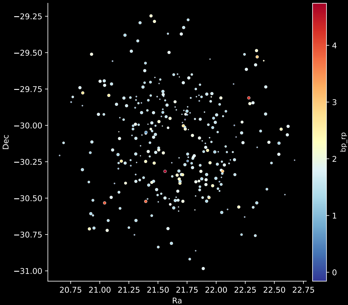
APOGEE DR17 Field: [SGRC3] Stars: 308
