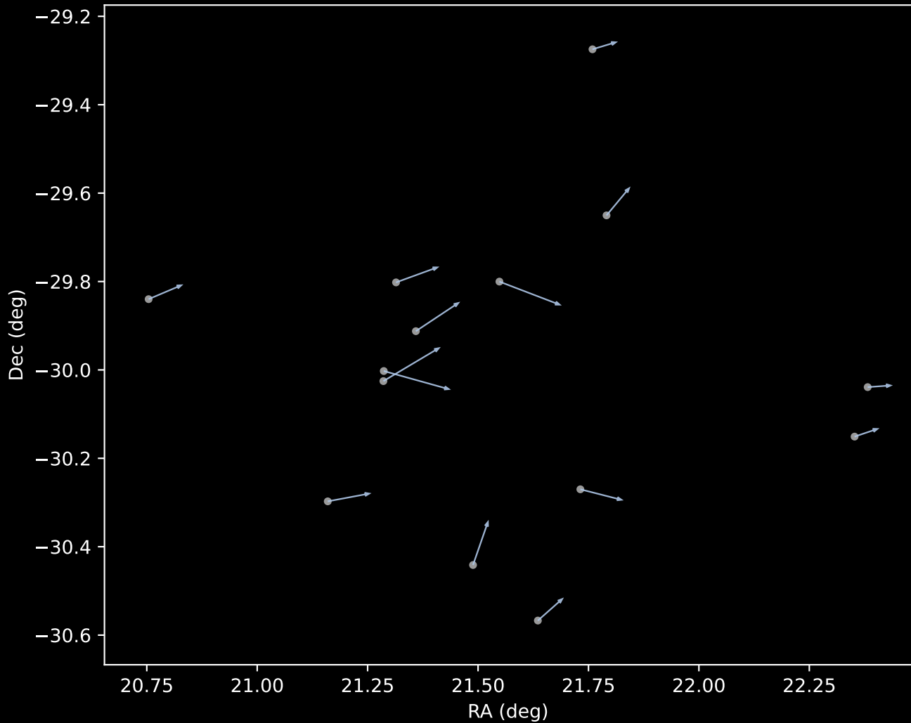
APOGEE DR17 Cluster 1 Proper Motion Vectors (n=14)
