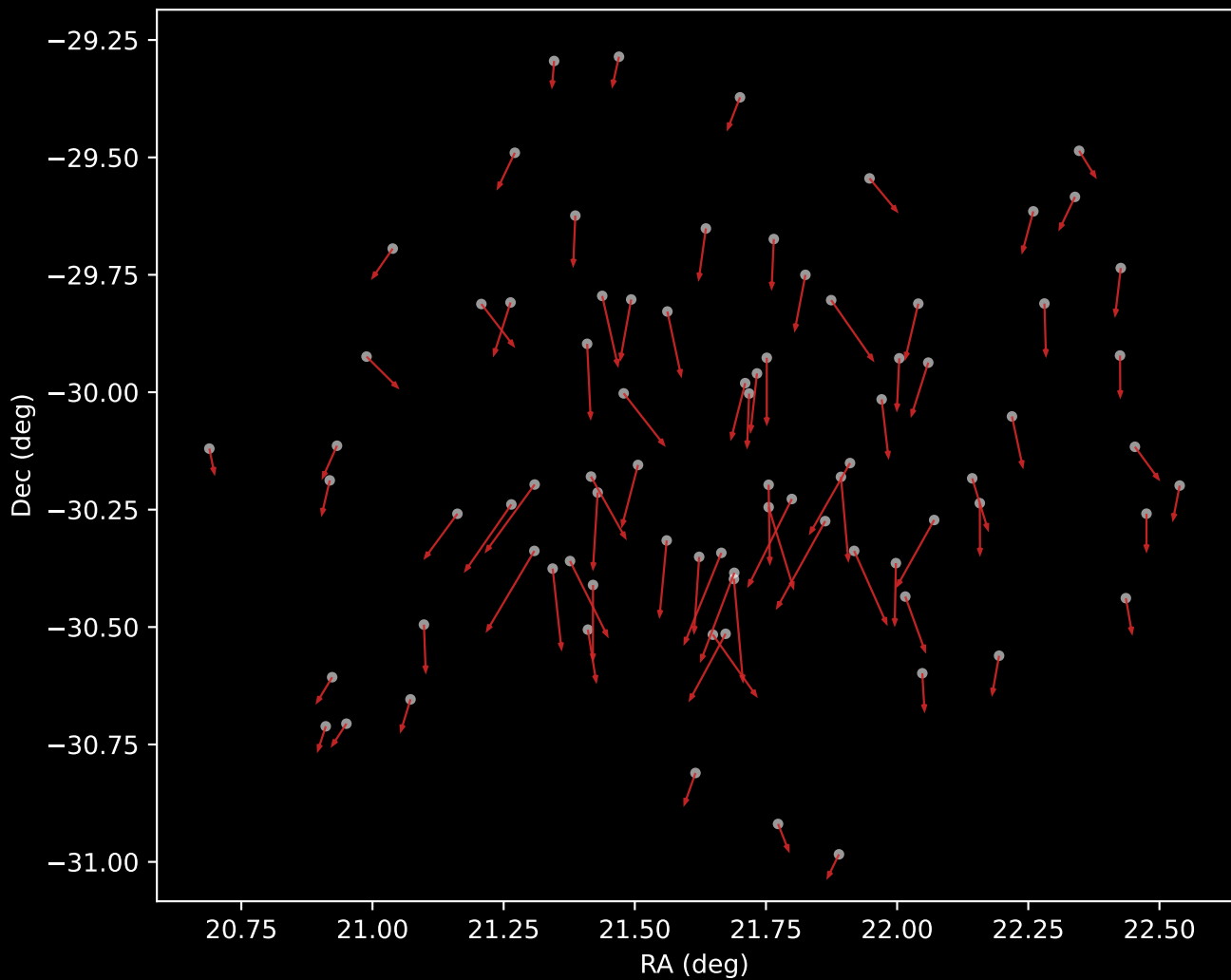
APOGEE DR17 Cluster 6 Proper Motion Vectors (n=81)
