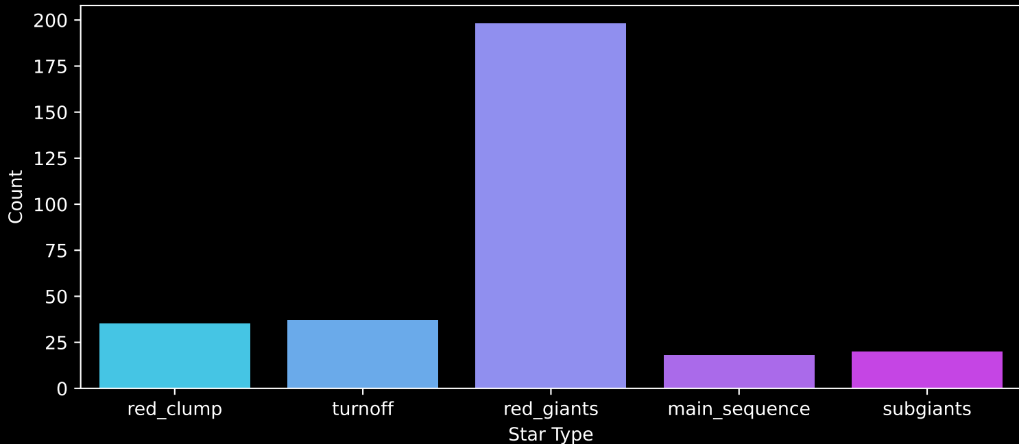
APOGEE DR17 Field: [SGRC3] Count plot of Star Type
